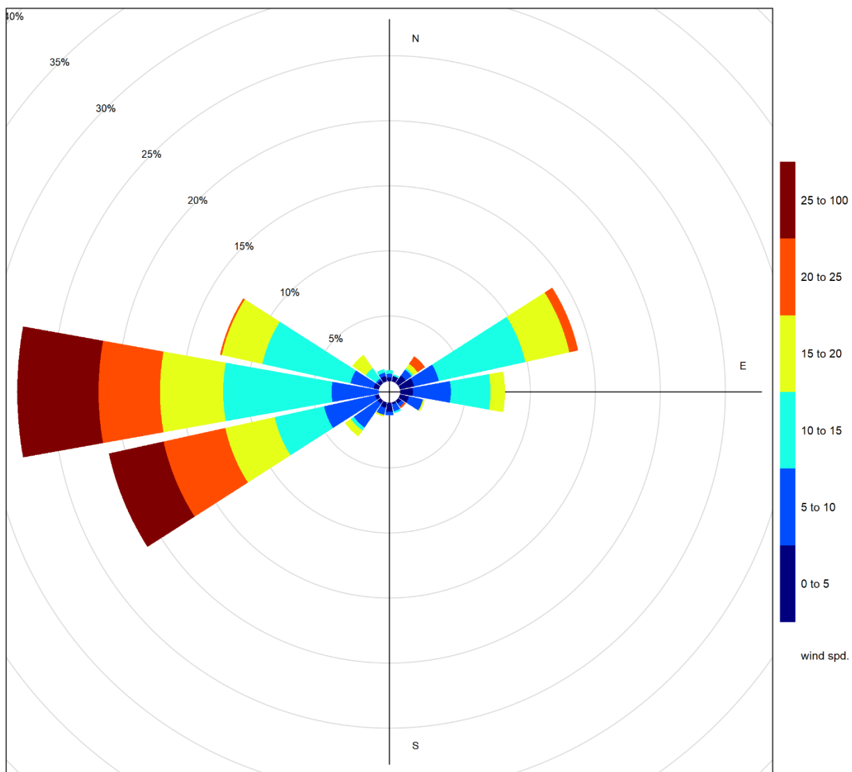
Figure 3-2 June 2021 wind rose for the Lagoon Station
