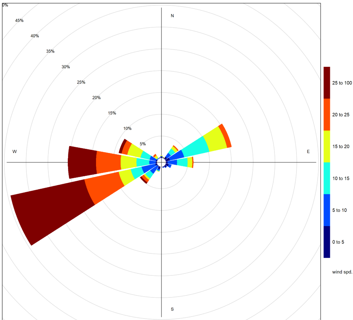
Figure 3-9 Wind rose for March 2022 recorded at the Lagoon Station
